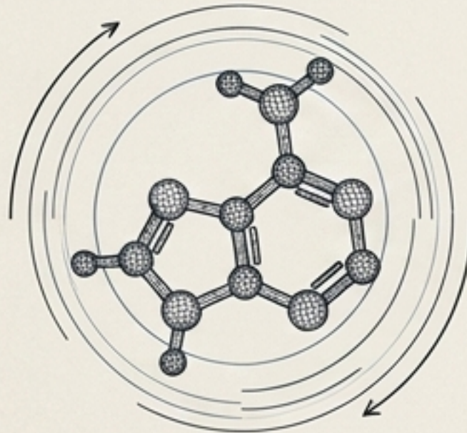
[Nucleobases (The information encoders)]
