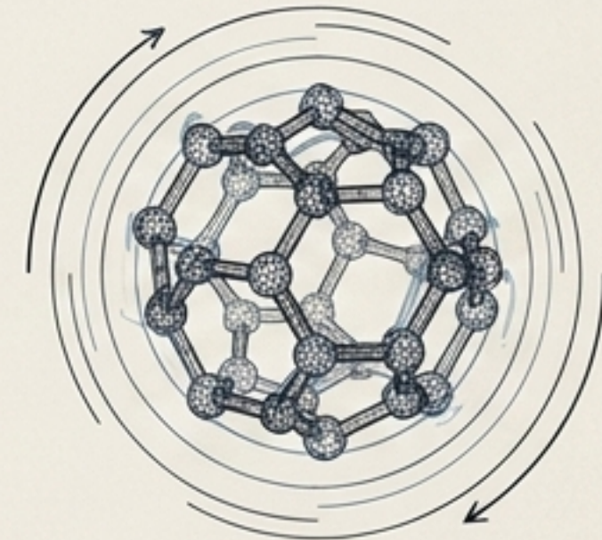
[Water Ice (The universal solvent)]
