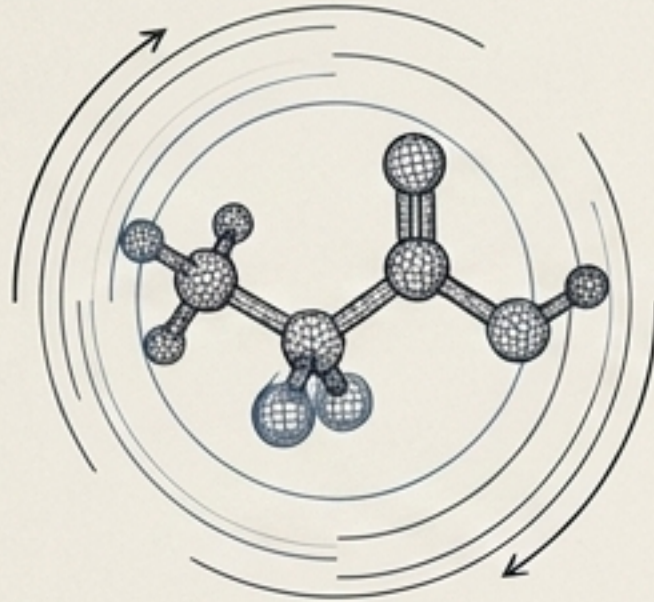
[Meteoritic Amino Acids (The structural scaffolding)]
