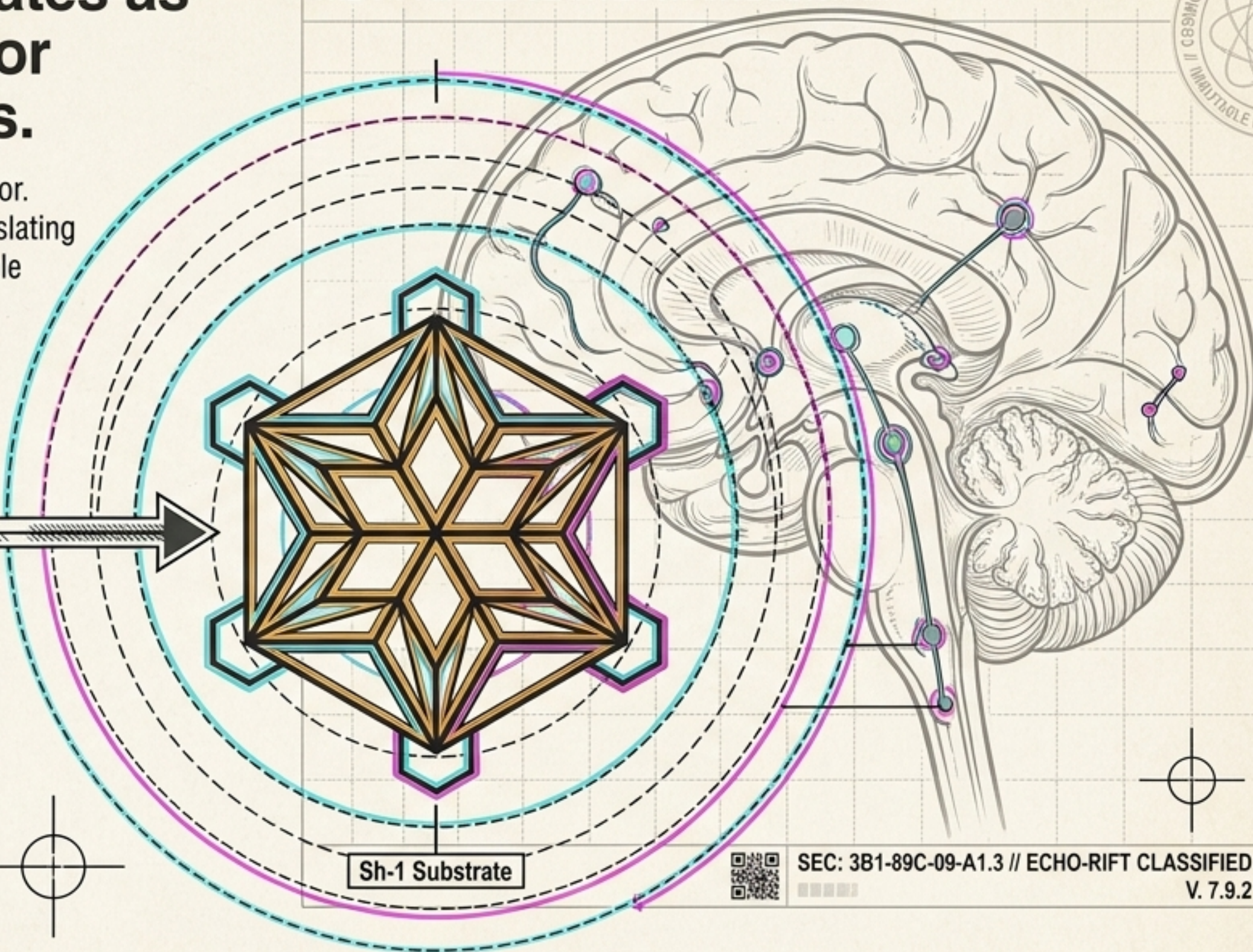
THE Sh-1 MOLECULAR RESONANCE DIAGRAM
