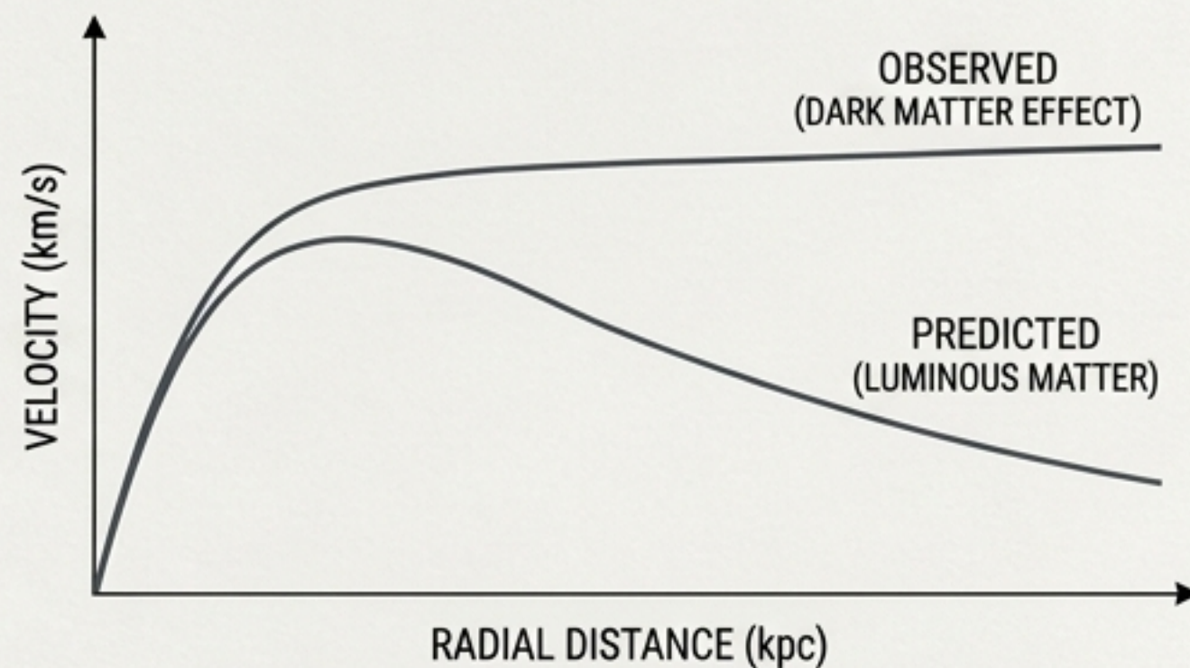
Galaxy Rotation Curve: Observed vs. Predicted
