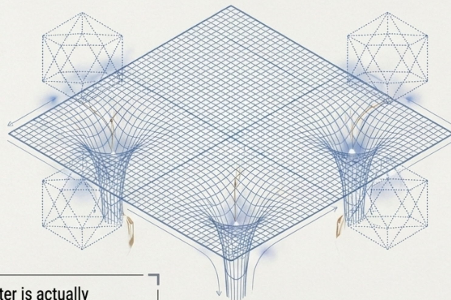
Multiversal Overlapping & Space-Time Distortion
