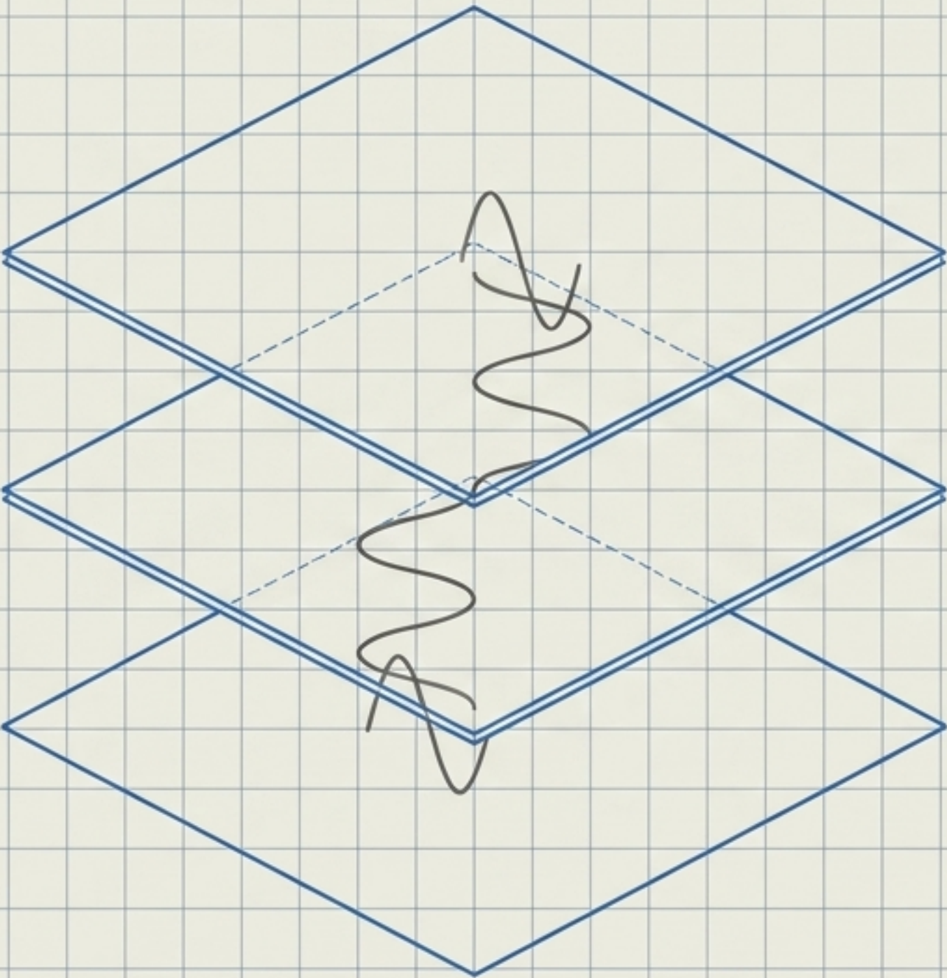
Kaluza-Klein Graviton Exchange
